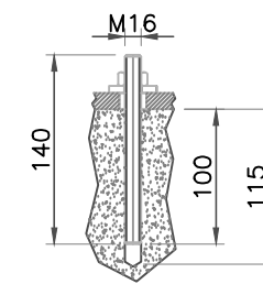
MECHANICAL ANCHORING DETAIL
